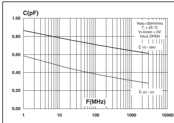
Figure 2. Line capacitance versus frequency (typical values) SATAULC6-2M6
