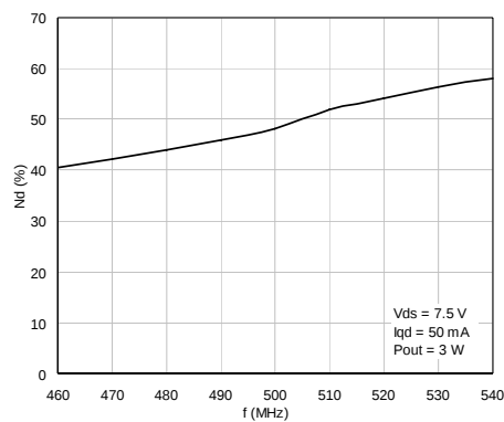
Figure 10. Efficiency vs Frequency
