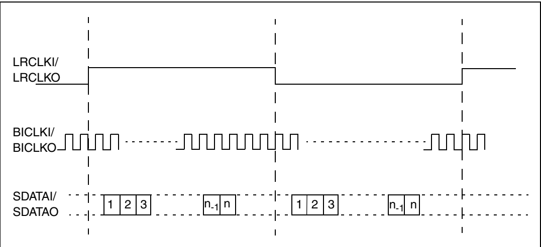
Figure 13. I 2 S
