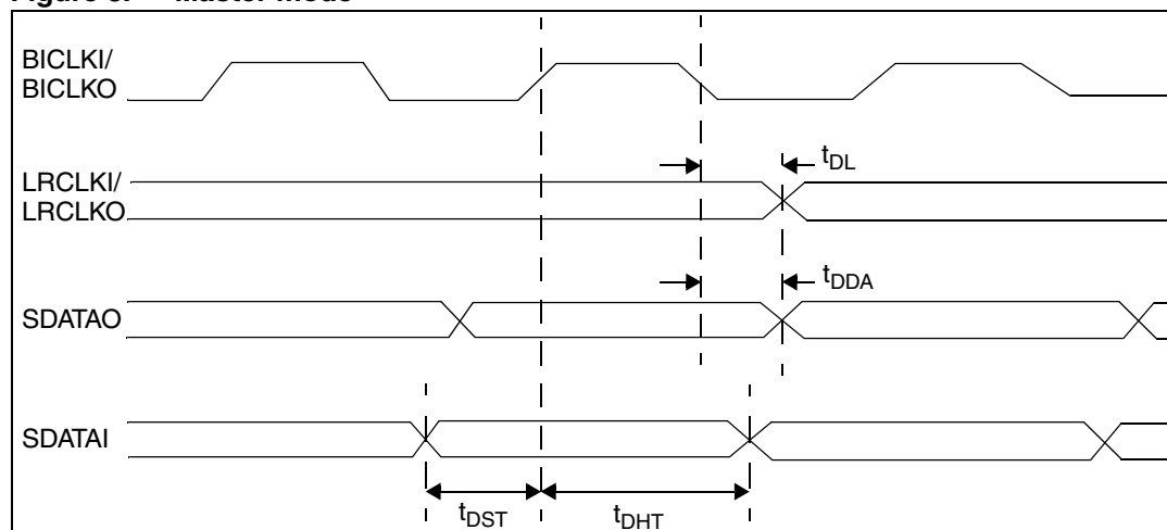
Figure 8. Master mode
