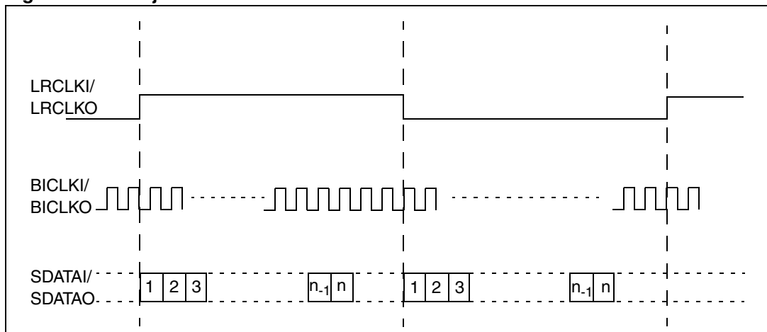
Figure 11. Left justified
