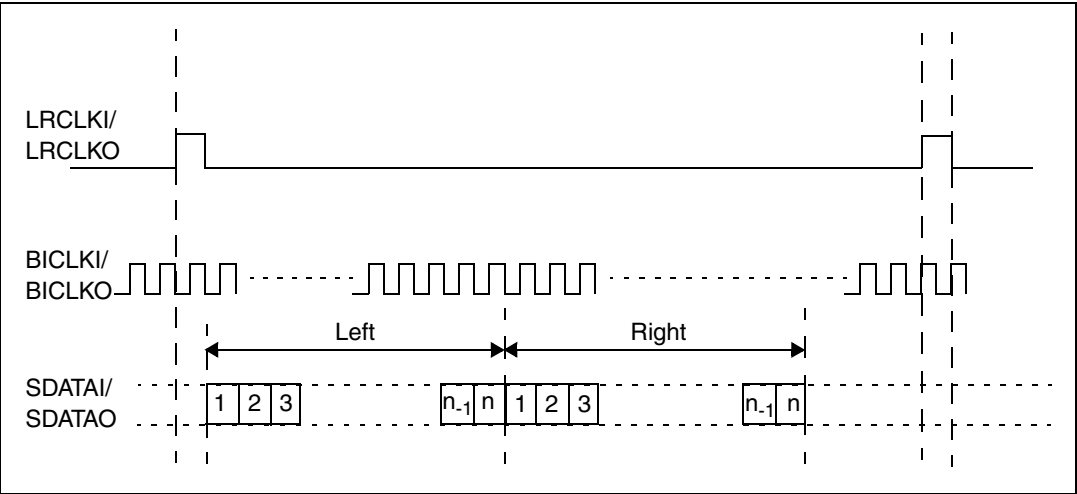
Figure 12. DSP
