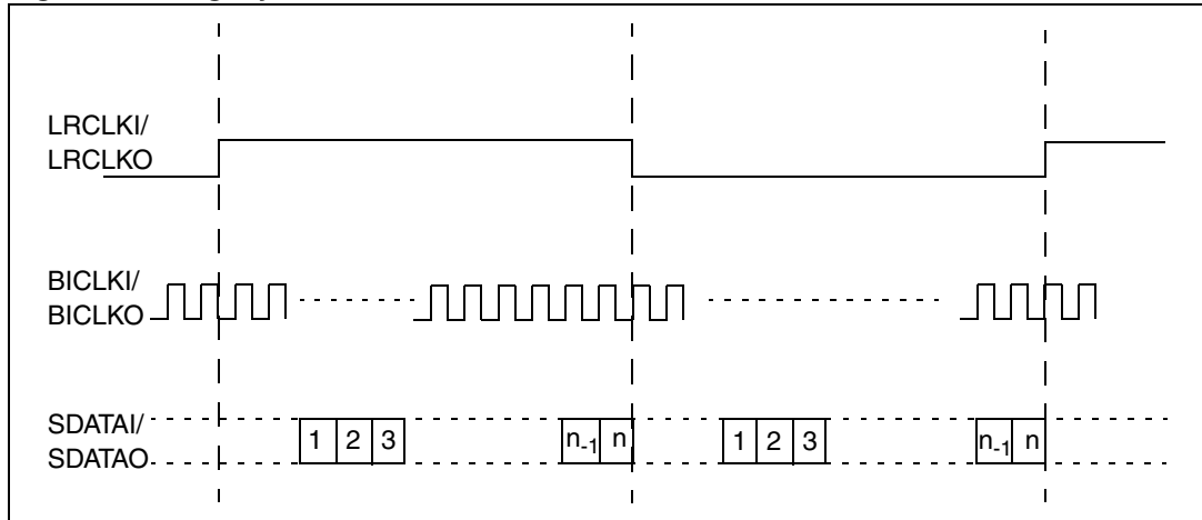
Figure 10. Right justified
