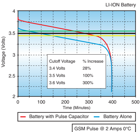
Figure 6b. Li-ION Battery at +0°C
