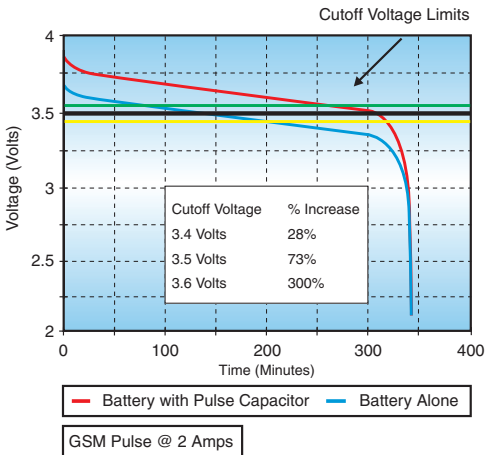
Figure 6a. Li-ION Battery at +25°C
