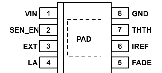
Package LJ, 8-Pin SOICN Pinout Drawing
