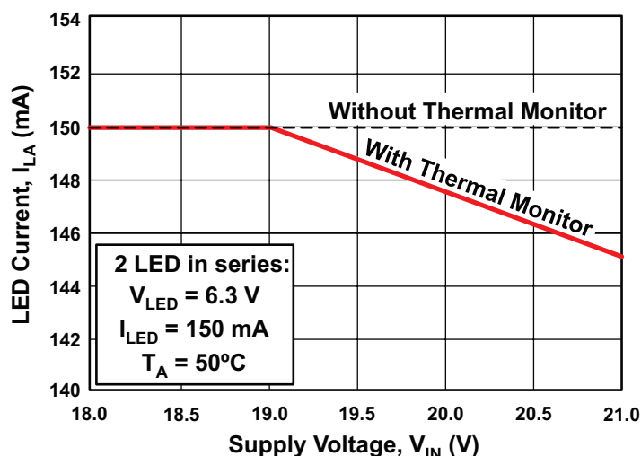
Figure 11: LED Current versus Supply Voltage
