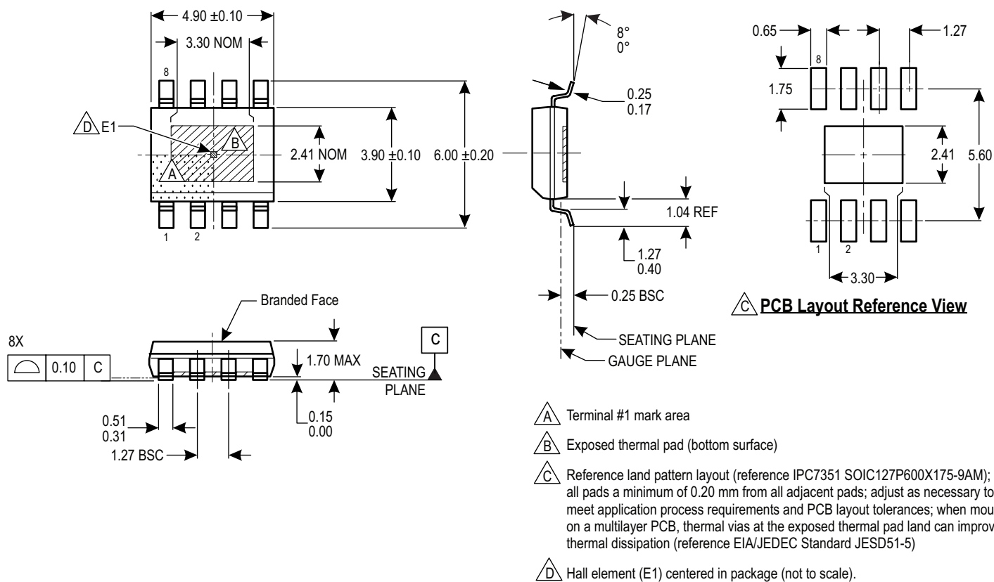
Figure 14: Package LJ, 8-Pin SOICN with Exposed Thermal Pad
