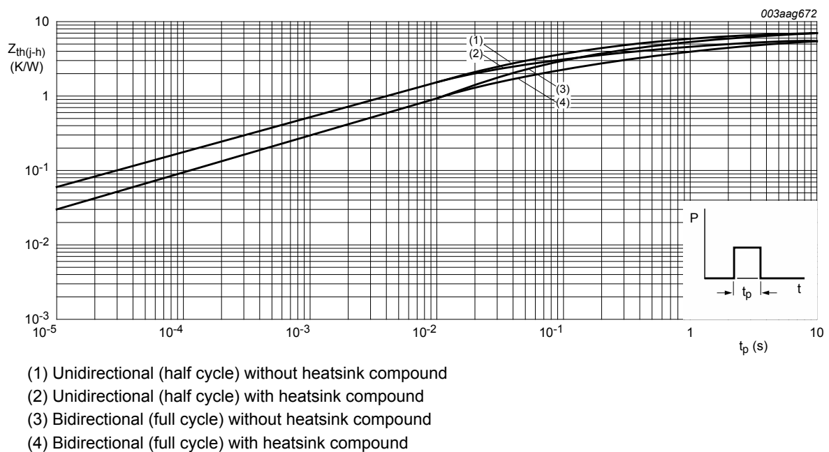
Fig. 6. Transient thermal impedance from junction to heatsink as a function of pulse duration
