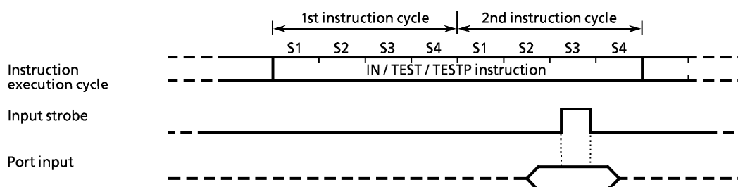
Figure 3-1. Input Timing
