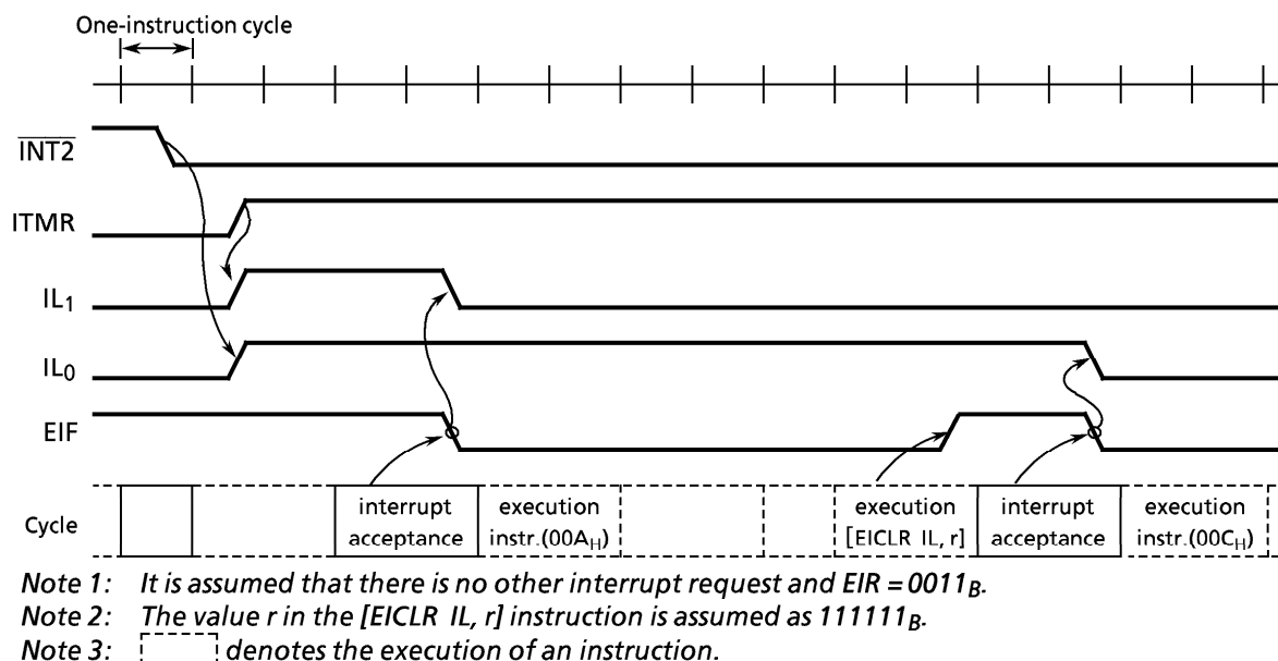
Figure 2-22. Interrupt Timing chart (Example)
