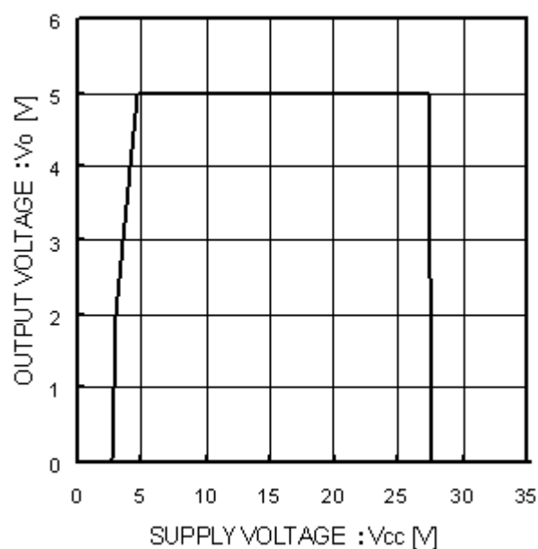
Fig.12 Overvoltage Operating ( I_o = 200 mA)
