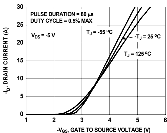
Figure 19. Transfer Characteristics
