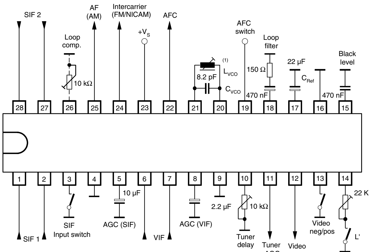
Figure 7-1. Test Circuit
