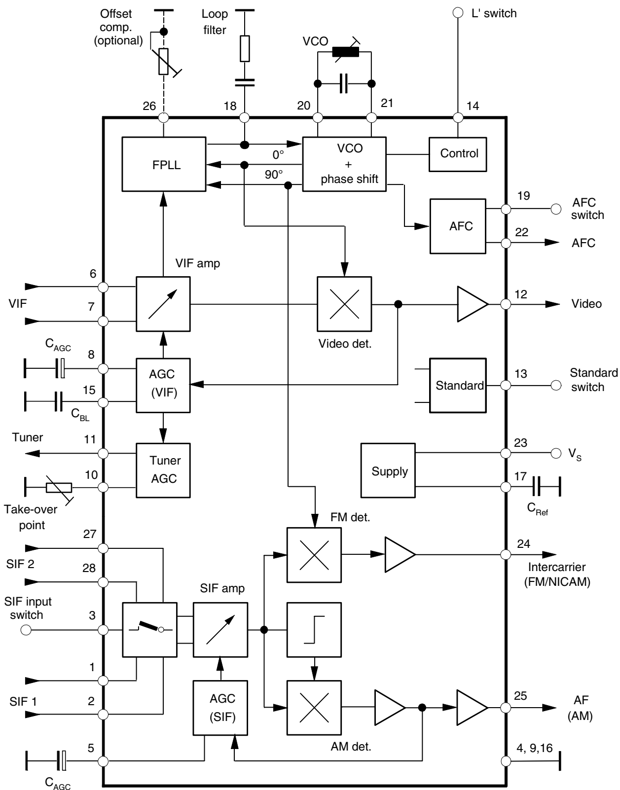
Figure 1-1. Block Diagram
