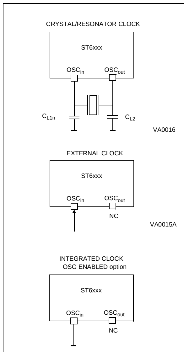
Figure 9. Oscillator Configurations
