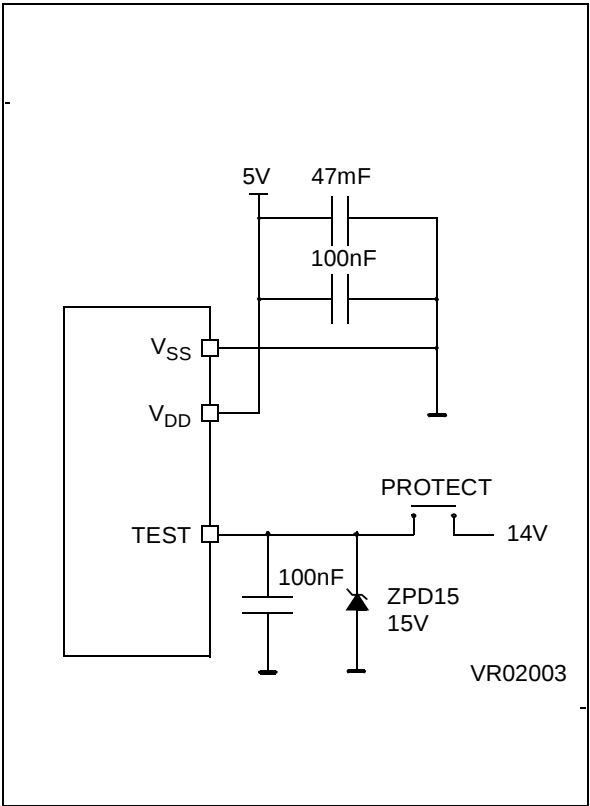
Figure 2. Programming Circuit
