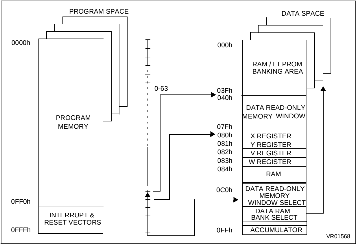
Figure 5. Memory Addressing Diagram
