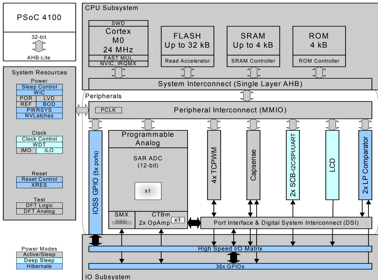
Figure 1. Block Diagram
