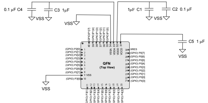
Figure 8. 40-pin QFN Example
