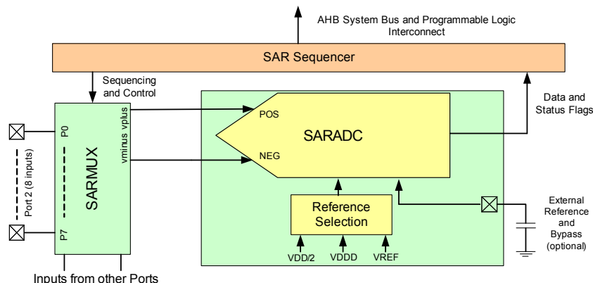
Figure 3. SAR ADC System Diagram
