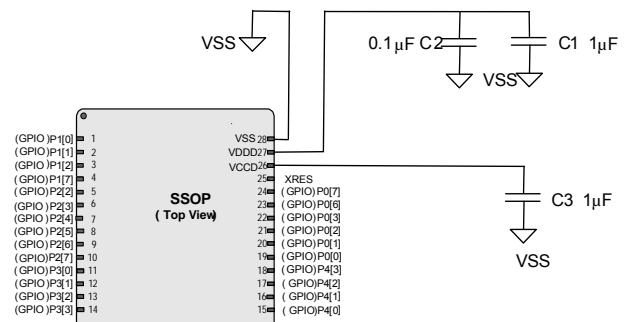
Figure 9. 28-SSOP Example
