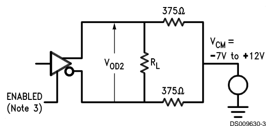
FIGURE 2. Driver V_{OD} with Varying Common Mode Voltage
