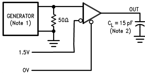
FIGURE 8. Receiver Propagation Delay Times
