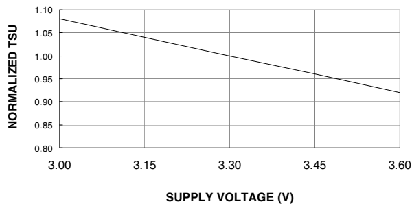
NORMALIZED T_{SU} VS. V_{CC}
