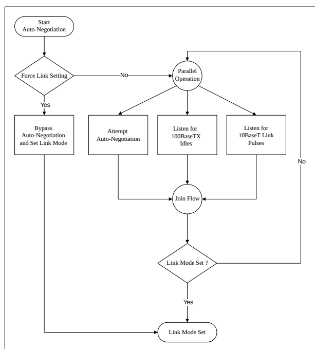
Figure 2. Auto-Negotiation
