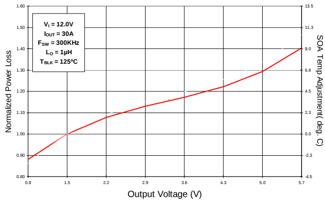
Fig. 4b: Power Loss vs. Output Voltage
