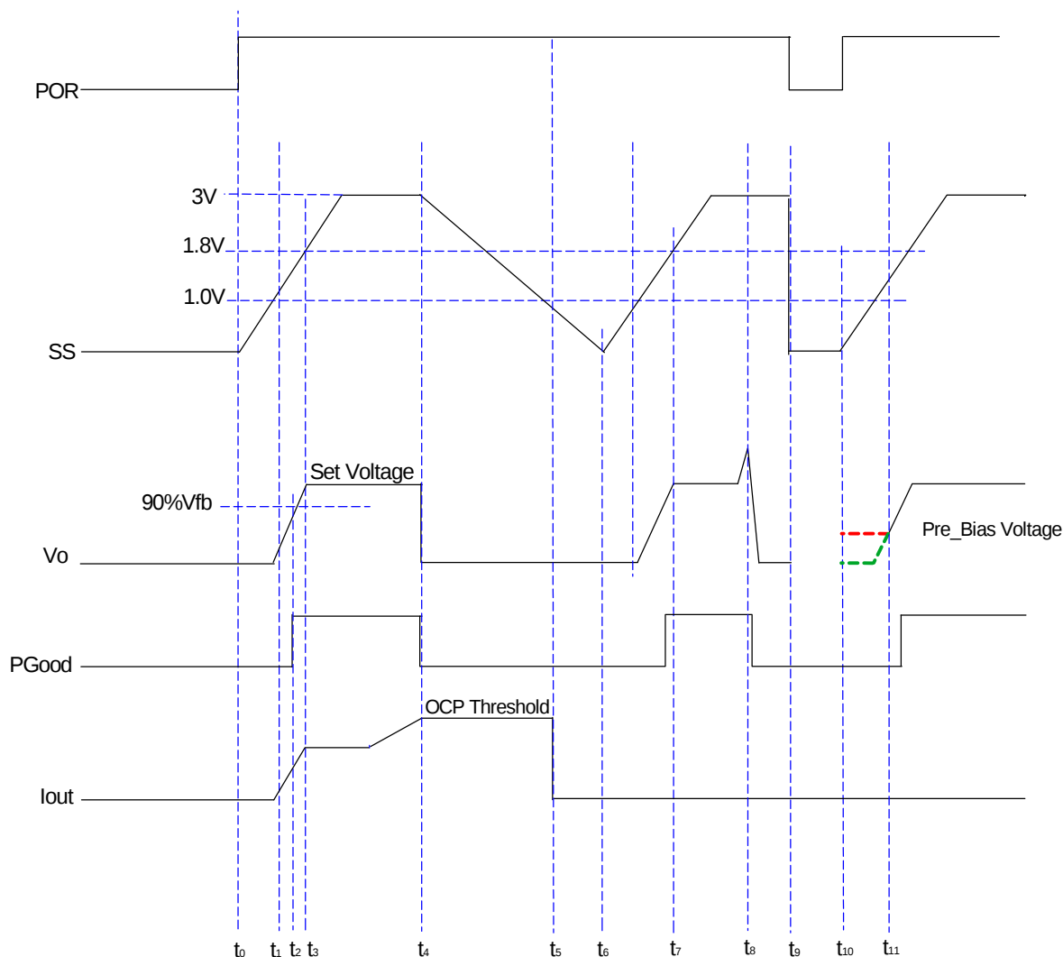
Fig. 15: Fault Conditions
