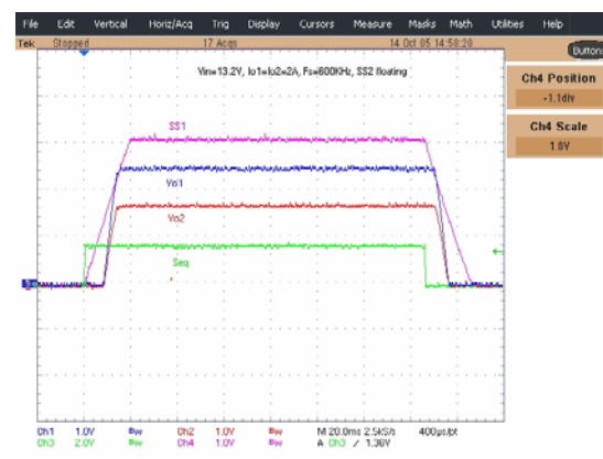
Fig. 13: Ratiometric Power up /down
