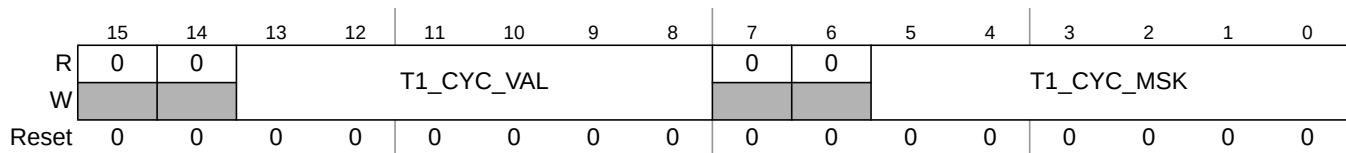
Figure 13-41. Timer 1 Cycle Set Register (T1CYSR)
