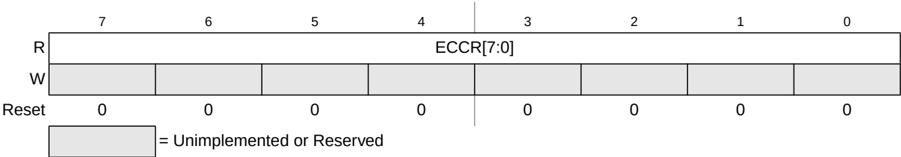
Figure 4-21. Flash ECC Error Results Low Register (FECCRLO)
