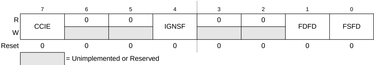
Figure 9-9. Flash Configuration Register (FCNFG)
