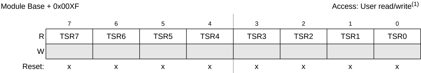
Figure 21-37. Time Stamp Register — Low Byte (TSRL)
