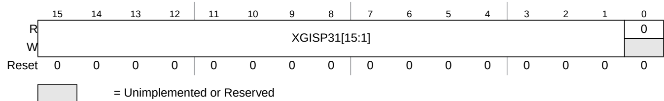
Figure 14-8. XGATE Initial Stack Pointer for Interrupt Priorities 3 to 1 (XGISP31)
