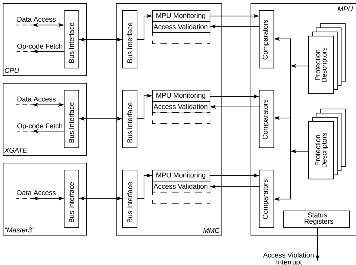
Figure 17-1. Block Diagram
