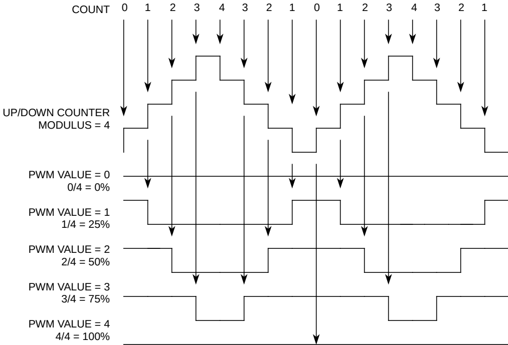
Figure 20-45. Center-Aligned PWM Pulse Width
