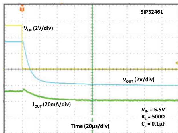
Fig. 43 - Turn-off Time
