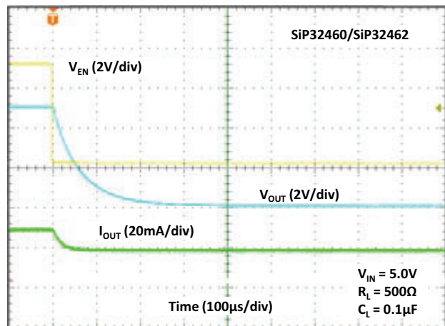
Fig. 38 - Turn-off Time
