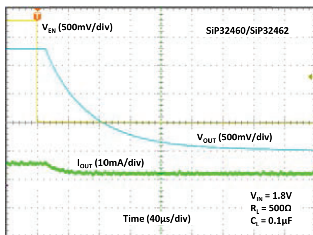
Fig. 36 - Turn-off Time
