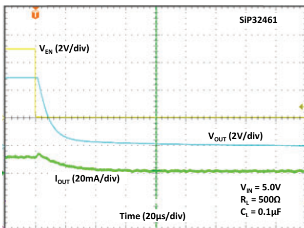
Fig. 40 - Turn-off Time
