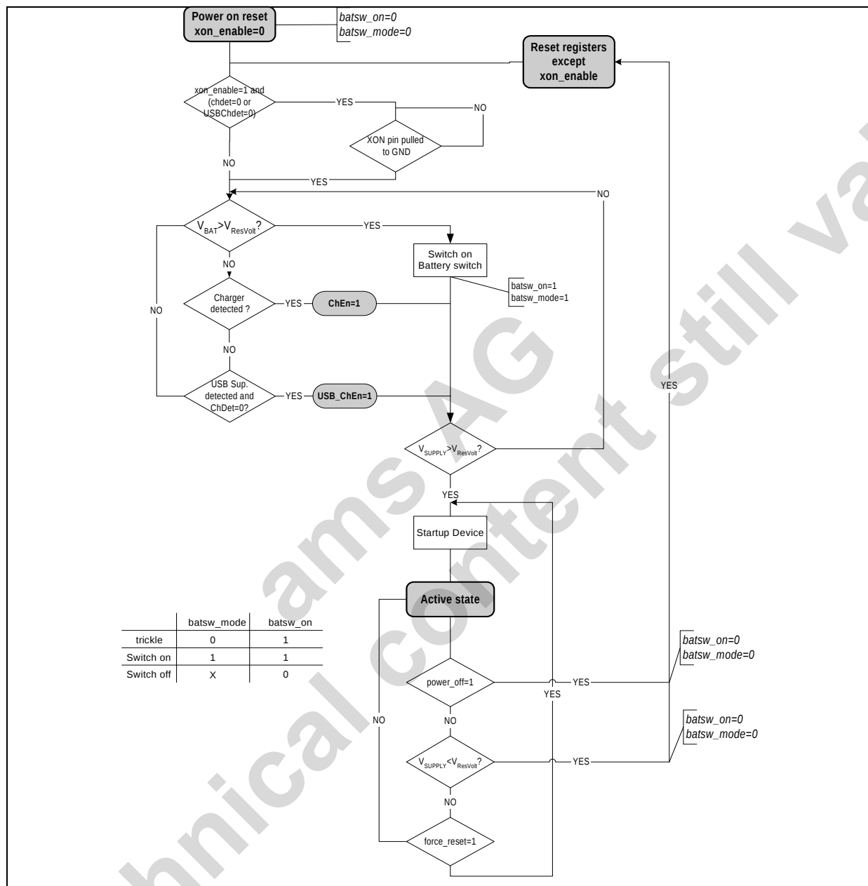
Figure 56. Startup flow chart
