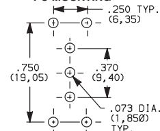
PC MOUNTING
