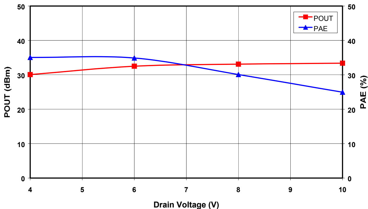
Figure 2. Saturated Output Power and Power Added Efficiency vs. Drain Voltage at f_0 = 4.5 GHz.
