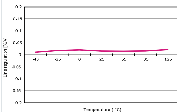
Figure 6. Line regulation vs. temperature
