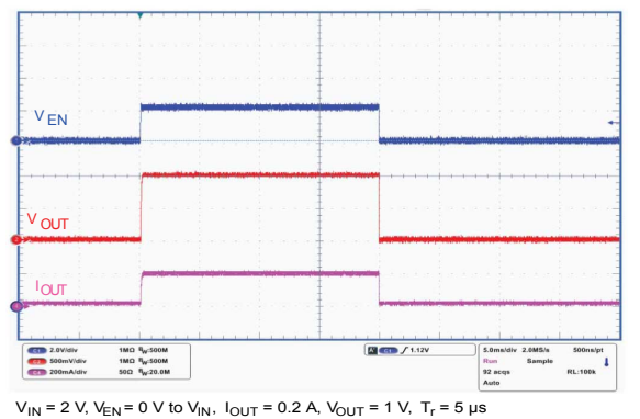
Figure 18. Enable startup ( V_{OUT} = 1\text{ V} )
