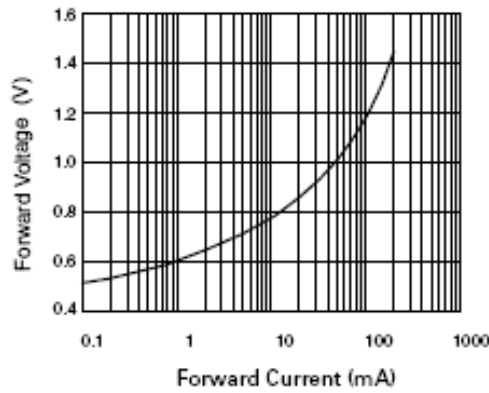
Forward Characteristics
