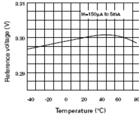
Temperature Drift
