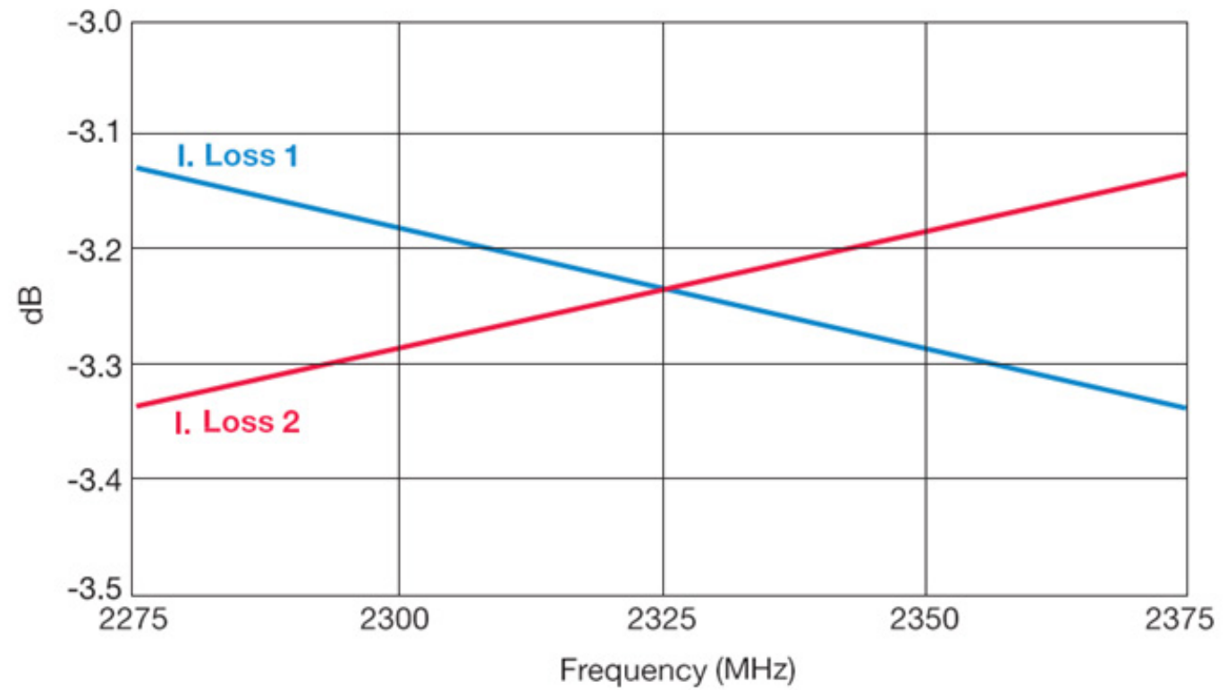
2325 ± 50MHZ DB0805A2325ASTR
