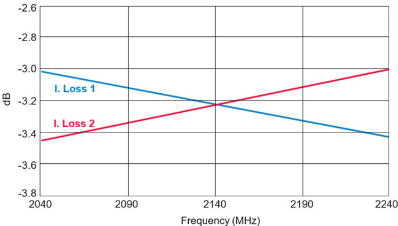
2140 ± 50MHZ DB0805A2140ASTR
