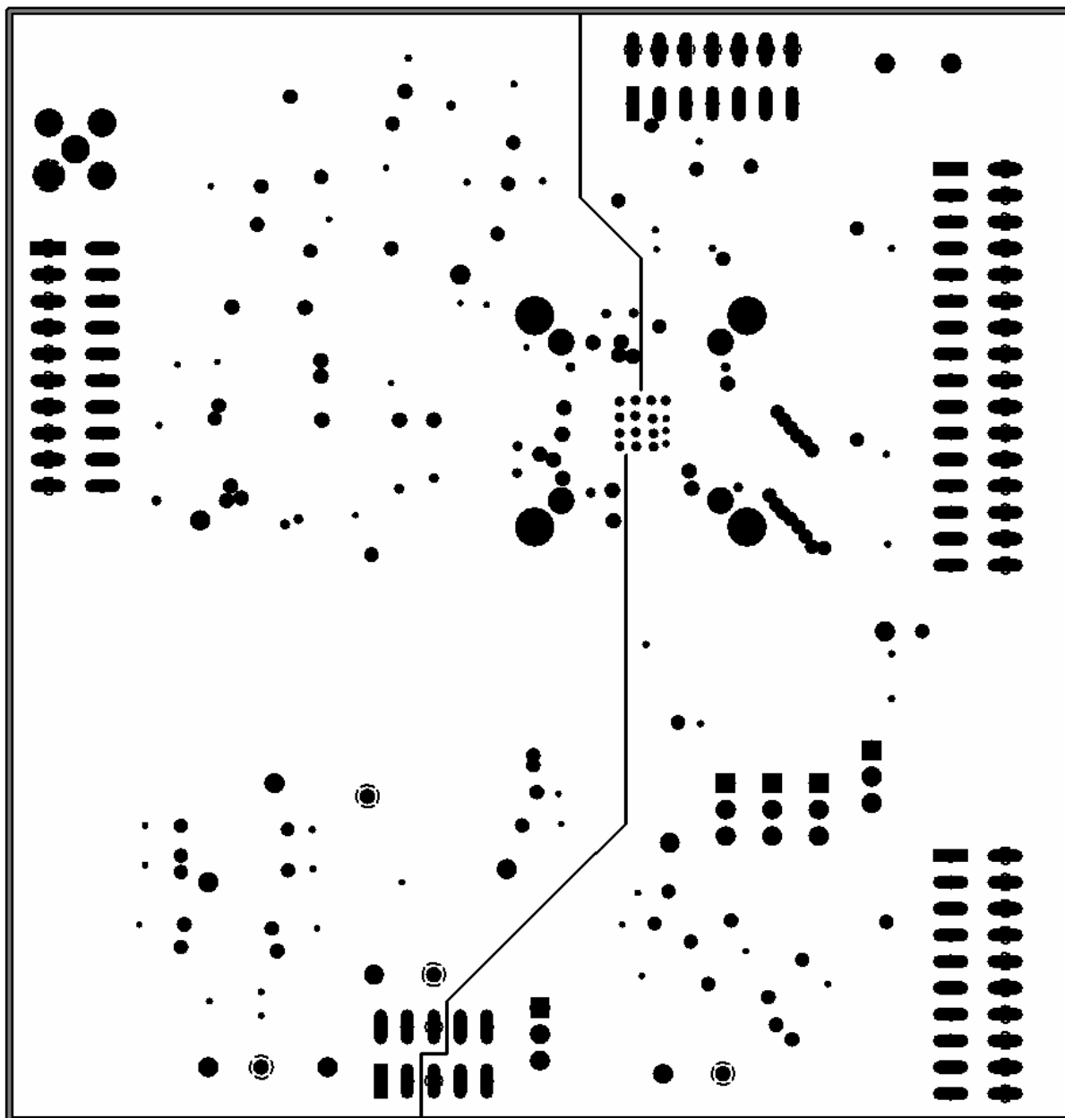
Figure 4-2. Ground Plane – Layer 2
