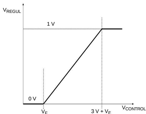
Figure 59. Correspondence between V_{\text{CONTROL}} and V_{\text{REGUI}}
