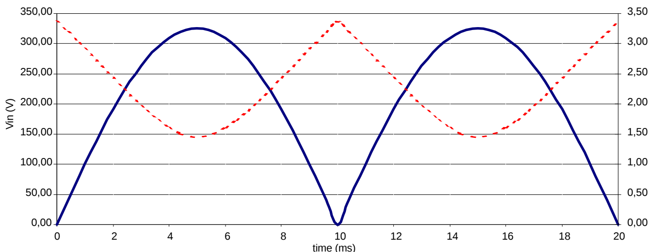
Figure 57. Input Voltage and On-time vs Time (example with F_{SW} = 100 kHz, P_{in} = 150 W, V_{AC} = 230 V, L = 200 \mu H)
