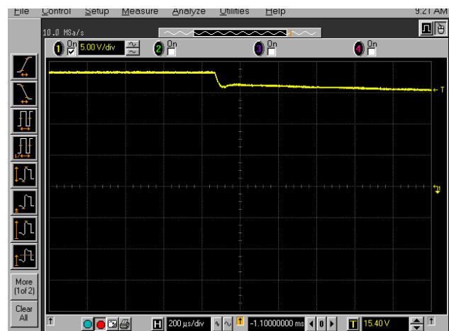
FIGURE 10. VLN TRANSITIONS FROM 18.3V TO 13.3V
