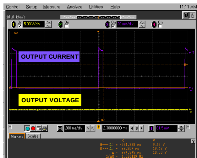
FIGURE 15. VLN SHORTED TO GND, 200mA 2
