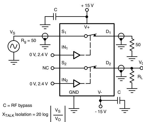
Fig. 4 - Channel-to-Channel Crosstalk
