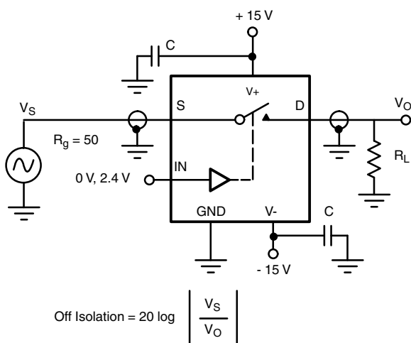
Fig. 3 - Off Isolation
