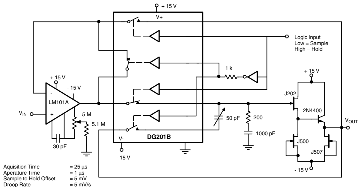
Fig. 6 - Sample-and-Hold
