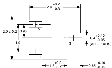
PACKAGE OUTLINE 33 (SOT-23)
