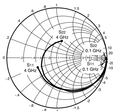
Coordinates in Ohms Frequency in GHz ( V_{CE} = 2.5\text{ V} , I_C = 1\text{ mA} )
