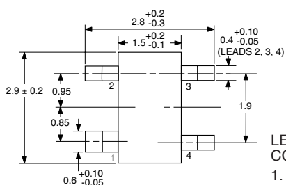
PACKAGE OUTLINE 39 (SOT-143)
