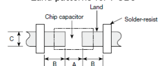
Land patterns for PCBs
