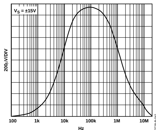
Figure 41. Band-Pass Response
