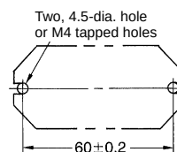
Mounting Holes
