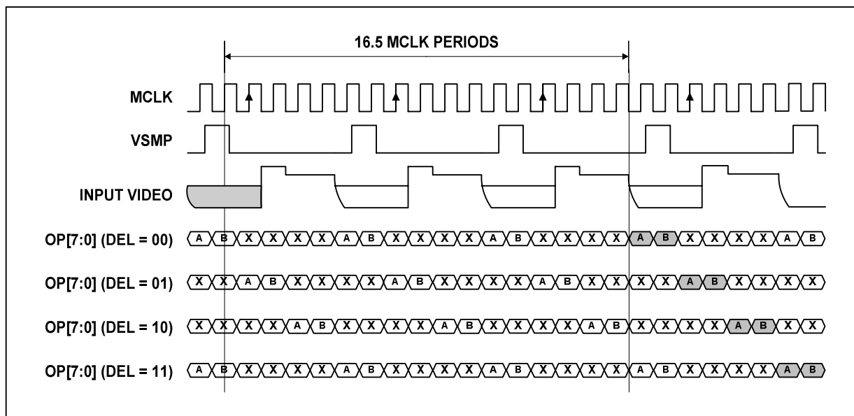
Figure 24 Mode 2 Operation
