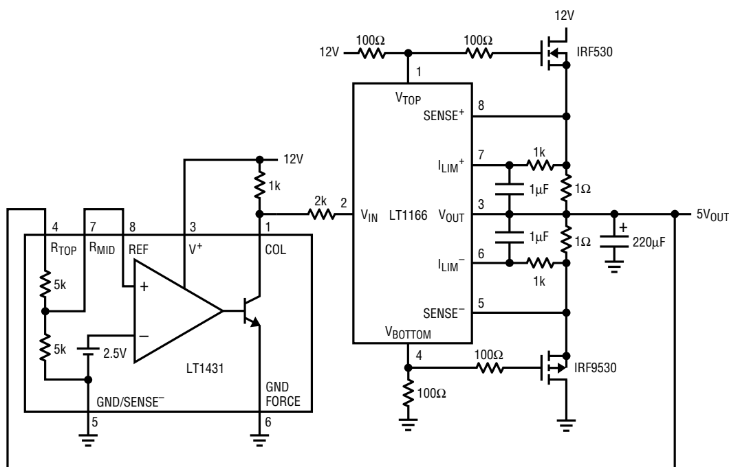
Figure 12. \pm 1A , 5V Voltage Reference
