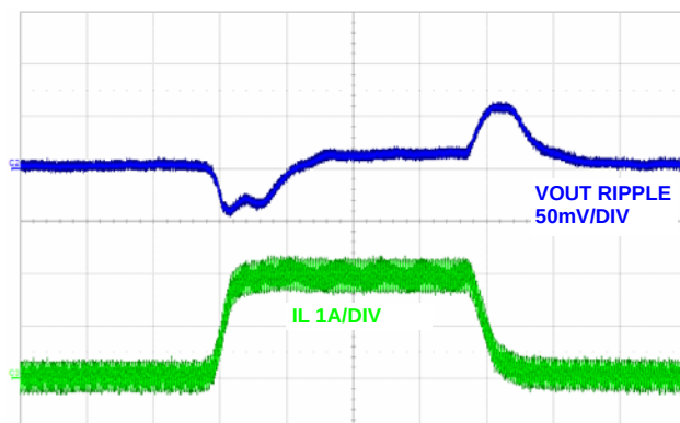
FIGURE 20. LOAD TRANSIENT (PWM), (50 \mu\text{s} /DIV)
