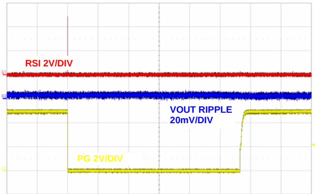
FIGURE 28. RSI RESET (ZOOM OUT), (200µs/DIV)
