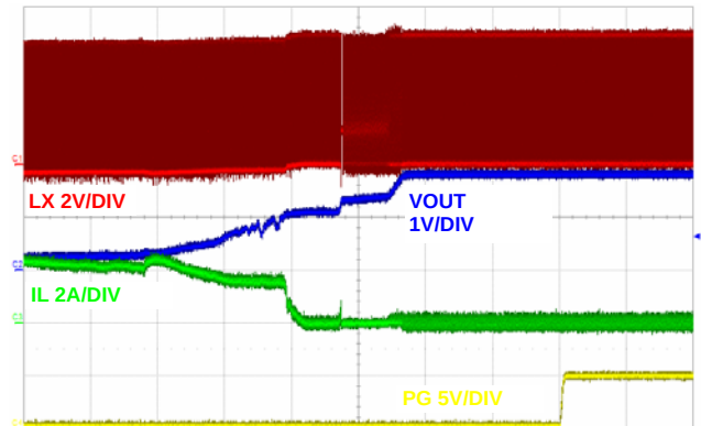
FIGURE 30. OUTPUT SHORT CIRCUIT RECOVERY, (500µs/DIV)
