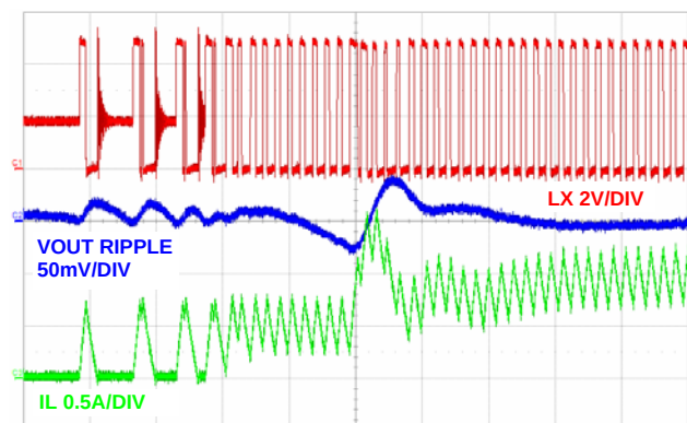
FIGURE 19. MODE TRANSITION DCM TO CCM, (50 \mu\text{s} /DIV)
