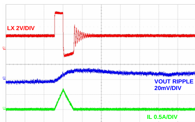
FIGURE 16. STEADY STATE OPERATION AT NO LOAD (PFM), (1 \mu\text{s} /DIV)
