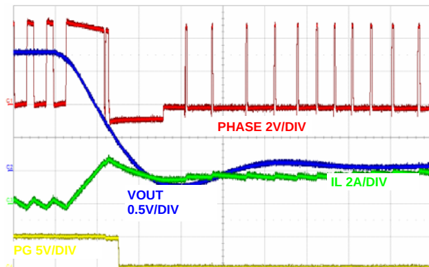
FIGURE 29. OUTPUT SHORT CIRCUIT, (500µs/DIV)
