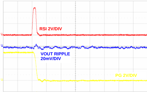
FIGURE 27. RSI RESET, (200µs/DIV)
