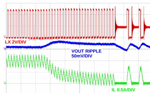
FIGURE 18. MODE TRANSITION CCM TO DCM, (5 \mu\text{s} /DIV)
