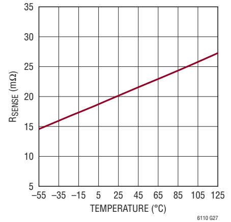
RSense vs Temperature
