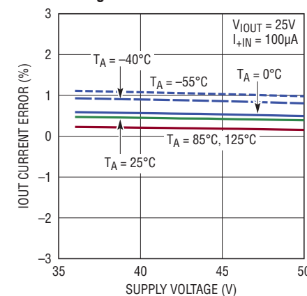
IOUT Current Error vs Supply Voltage
