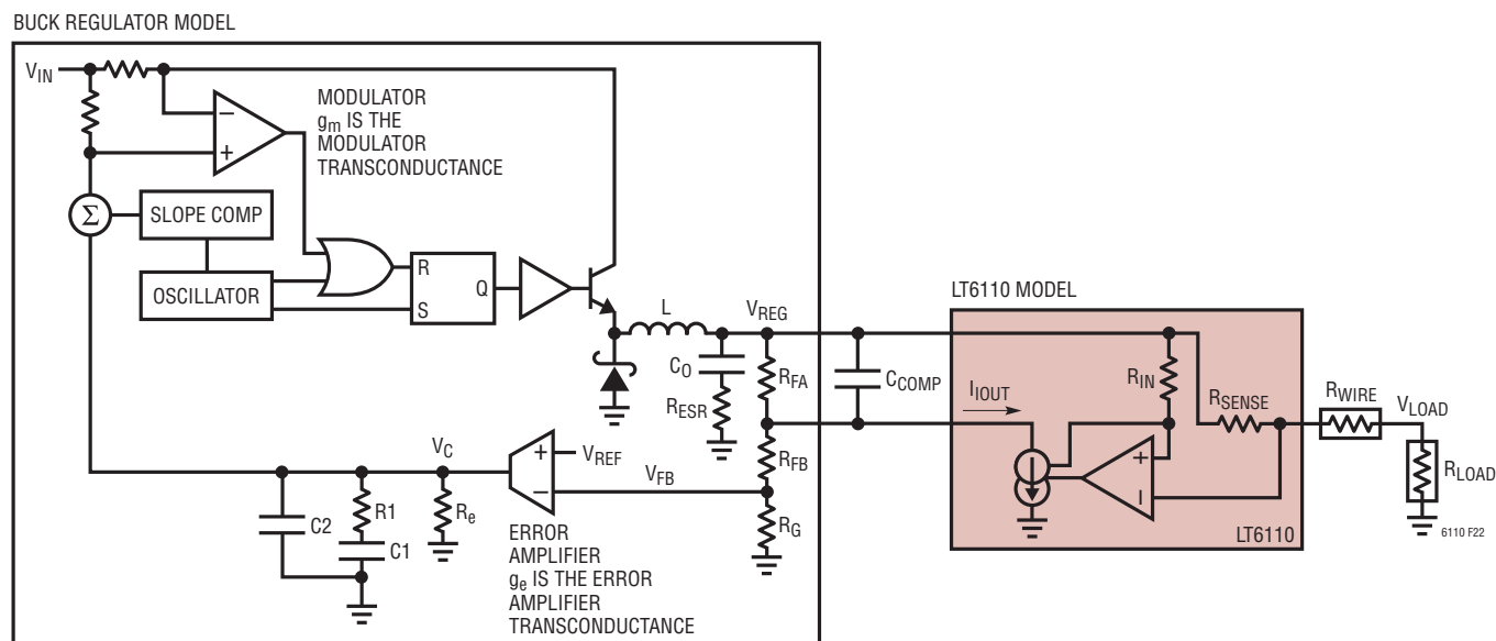
Figure 22. A Small-Signal Model: Current Mode Buck Regulator with an LT6110
