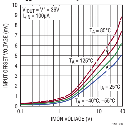
V_{OS} vs IMON Voltage
