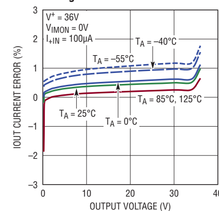
IOUT Current Error vs Output Voltage
