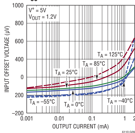
V_{OS} vs +IN Current
