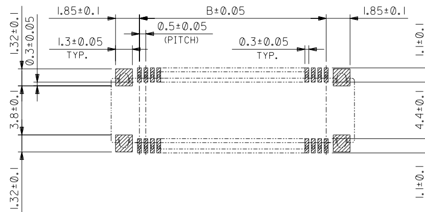
RECOMMENDED PCB PATTERN LAYOUT (SCALE:5-1)
