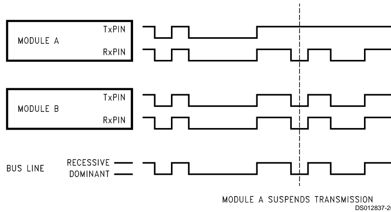
FIGURE 18. CAN Message Arbitration
