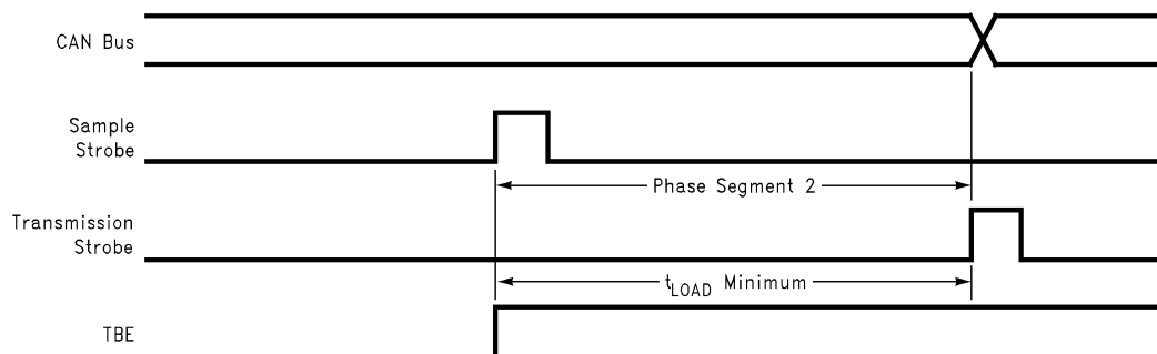
FIGURE 16. TBE Timing
