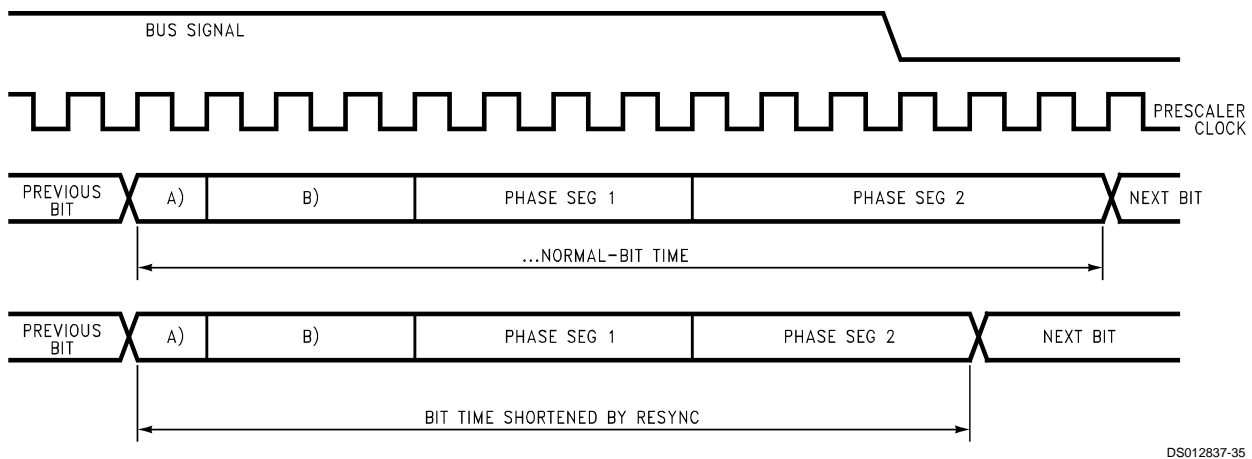
FIGURE 30. Resynchronization 2
