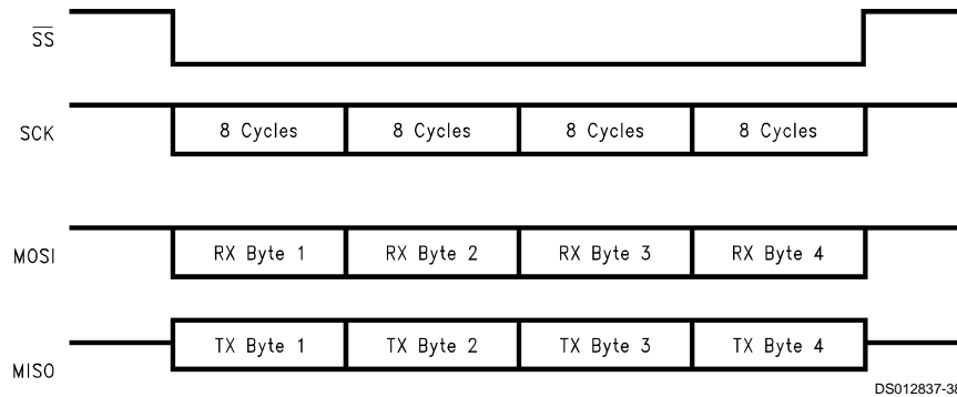
FIGURE 36. SPI Transmission Example
