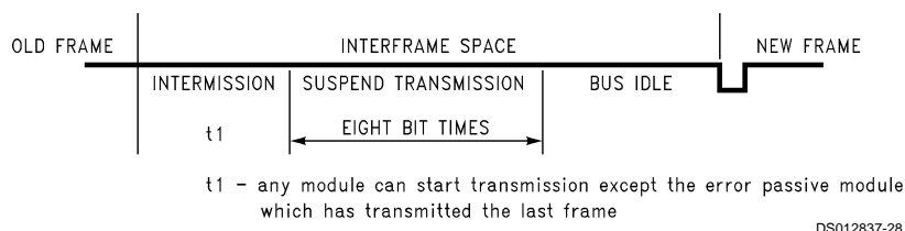
FIGURE 23. Interframe Space for Nodes Which Are Error Passive and Have Been Transmitter for the Last Frame
