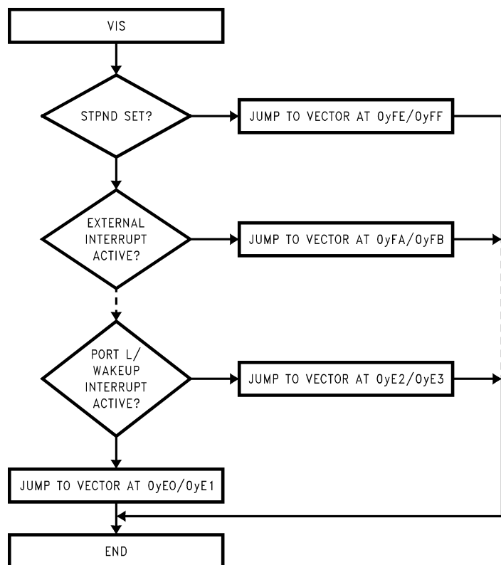
FIGURE 33. VIS Flowchart
