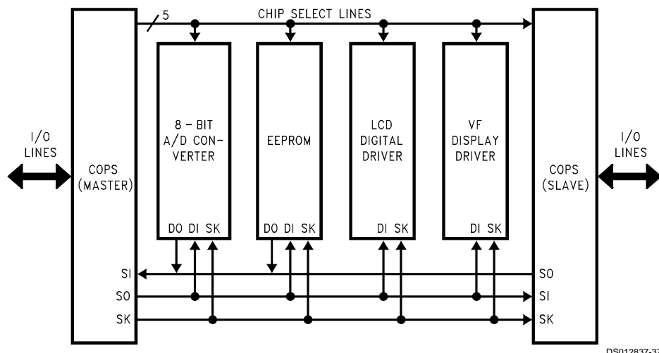
FIGURE 35. MICROWIRE/PLUS Application
