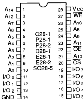
DIP/SOJ/SOIC TOP VIEW
