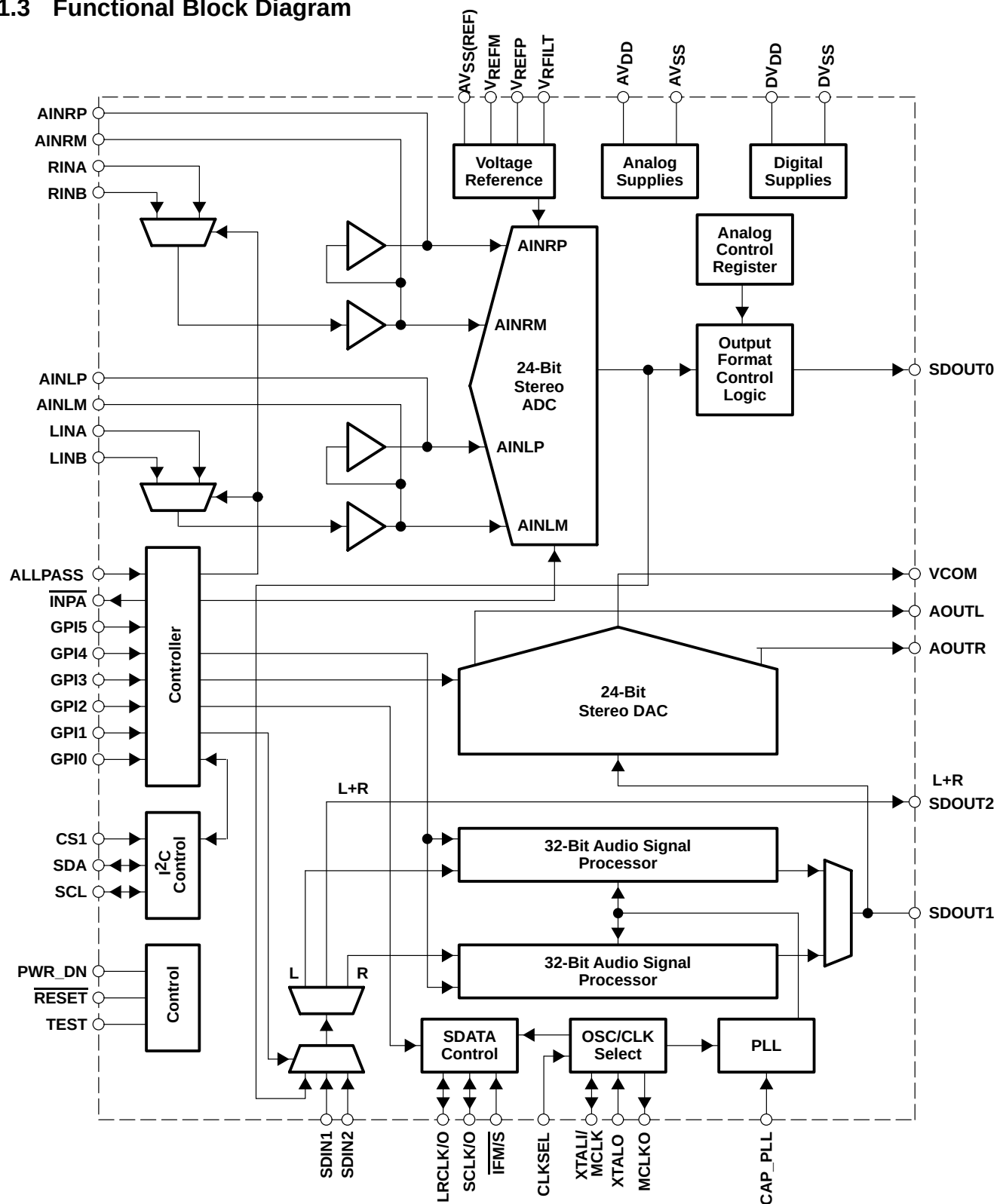
Figure 1-1. TAS3004 Block Diagram
