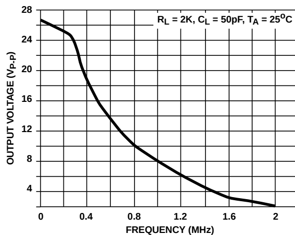
FIGURE 16. V_{OUT} MAX (UNDISTORTED SINEWAVE OUTPUT) vs FREQUENCY
