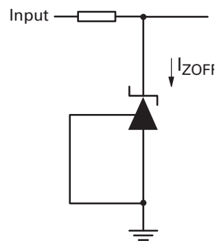
Fig 3 - Test circuit for for OI state current †
