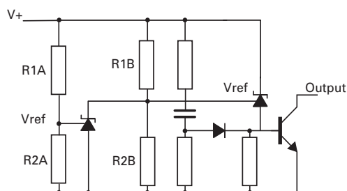
Series regulator
