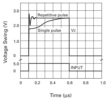
Pulse Response
