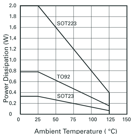
Power Dissipation Derating
