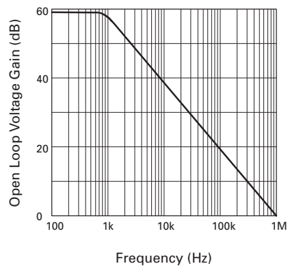
Gain v Frequency
