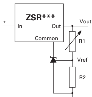
Shunt regulator
