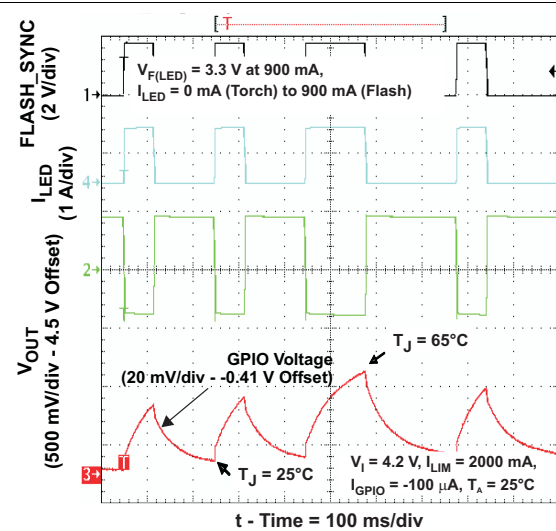
Figure 52. Junction Temperature Monitoring
