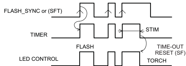
Figure 21. Level Sensitive Safety Timer (Normal Operation + Time-Out)
