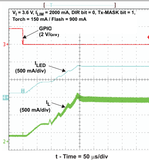
Figure 51. TX-Masking Operation
