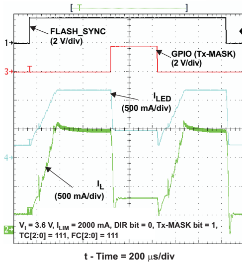
Figure 49. TX-Masking Operation
