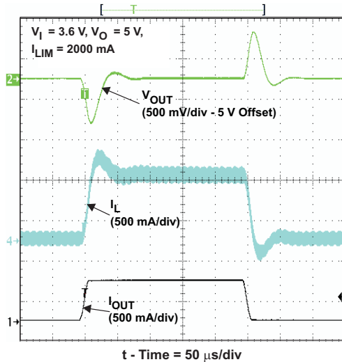
Figure 43. Voltage Mode Load Transient Response
