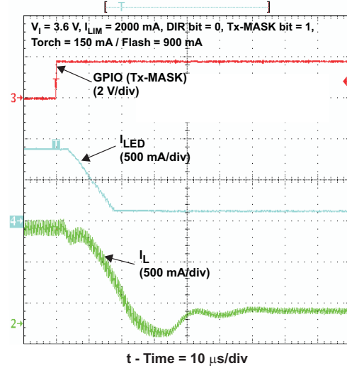
Figure 50. TX-Masking Operation
