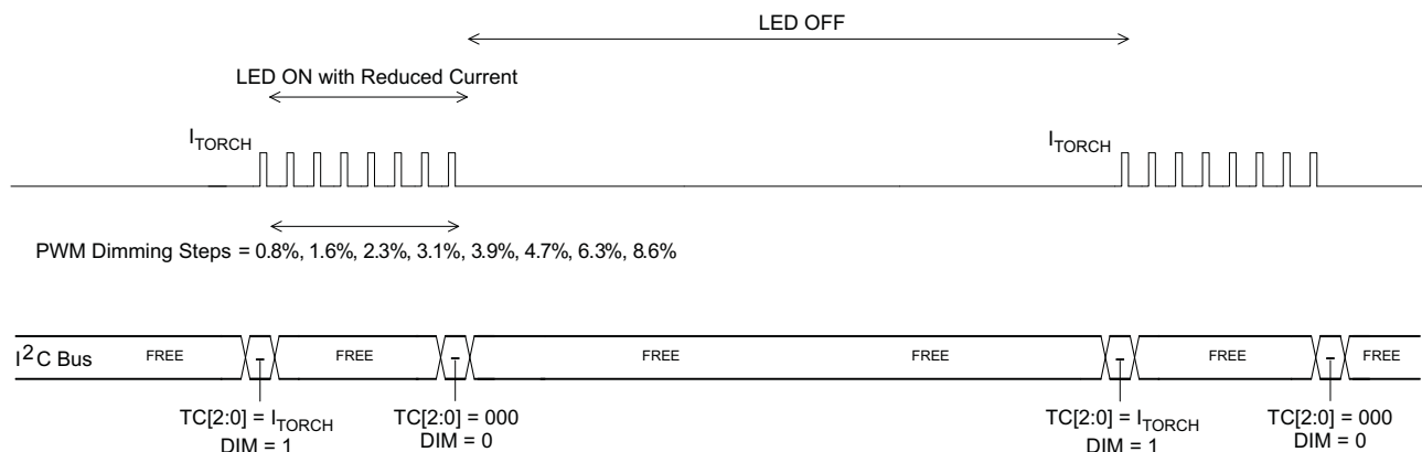
Figure 27. White LED Blinking Control
