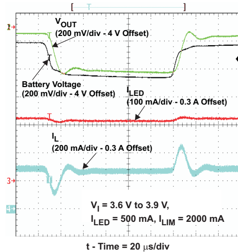
Figure 44. Down-Mode Line Transient Response
