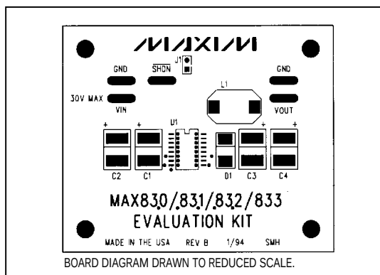
Figure 2. MAX831 EV Kit Component Placement Guide—Component Side
