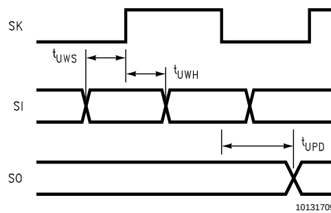
FIGURE 3. MICROWIRE/PLUS Timing
