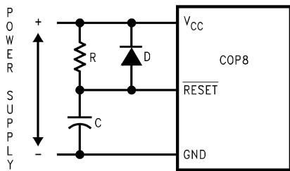
FIGURE 9. Reset Circuit Using External Reset
