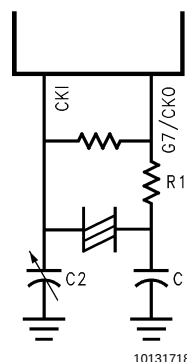
Without On-Chip Bias Resistor
