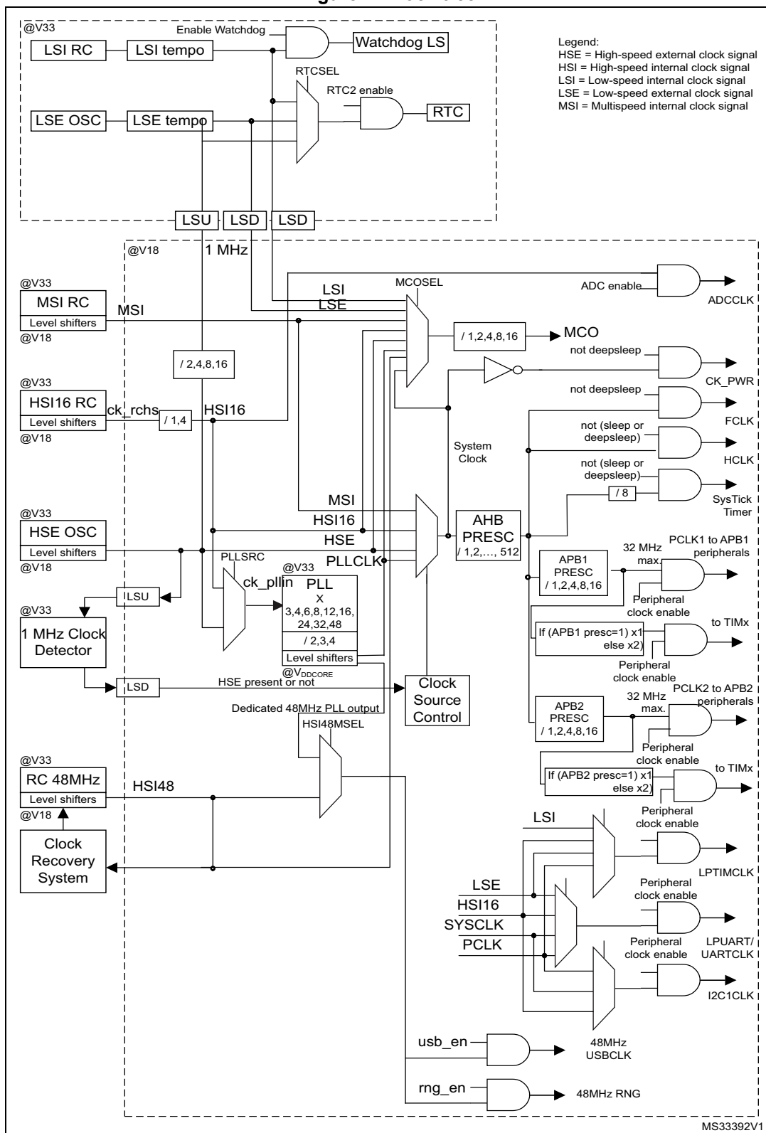
Figure 2. Clock tree
