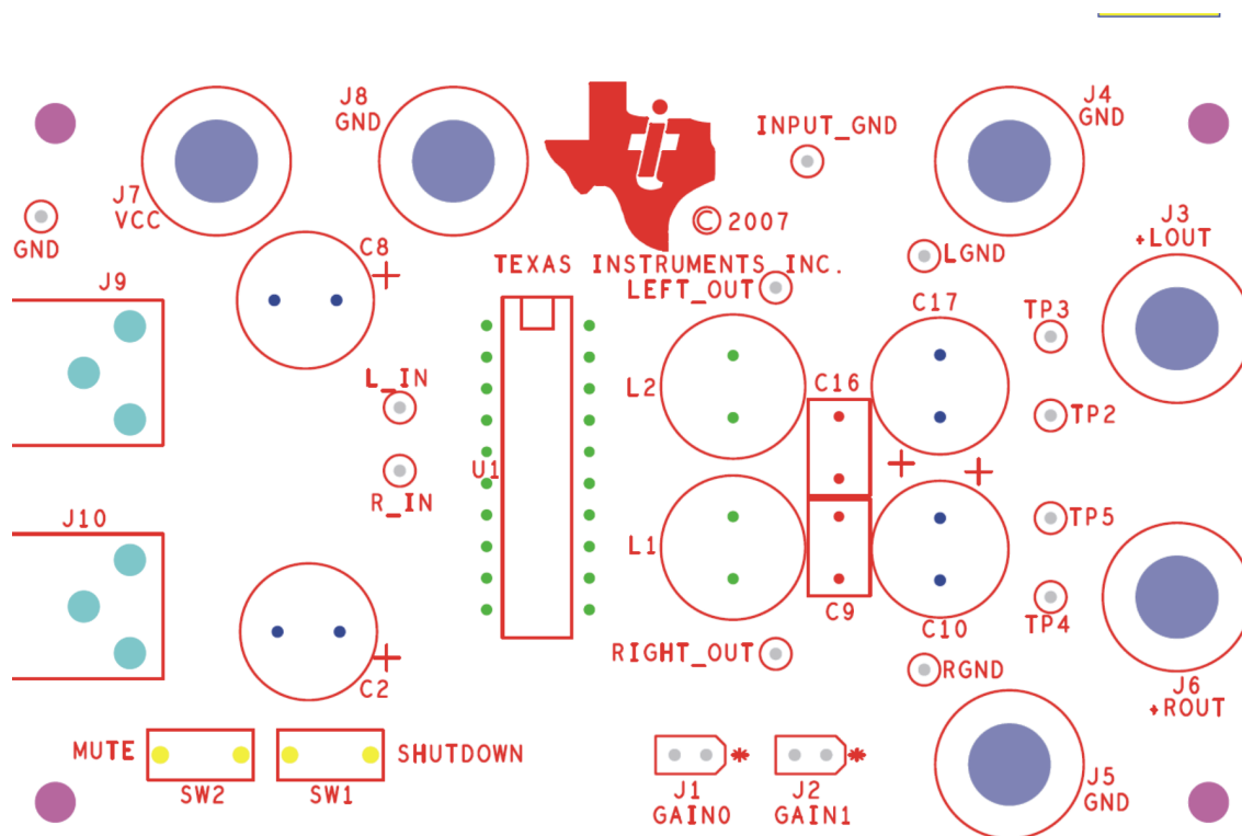
Figure 4. TPA3122D2 EVM – Top Side Layout
