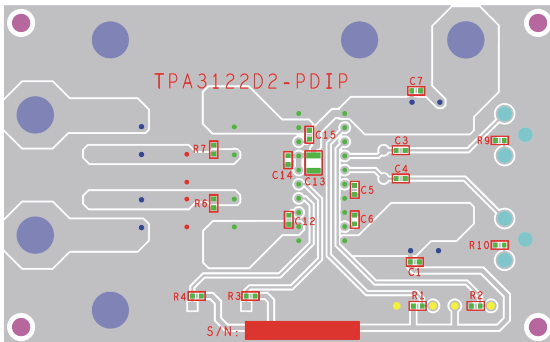
Figure 5. TPA3122D2 EVM – Bottom Side Layout
