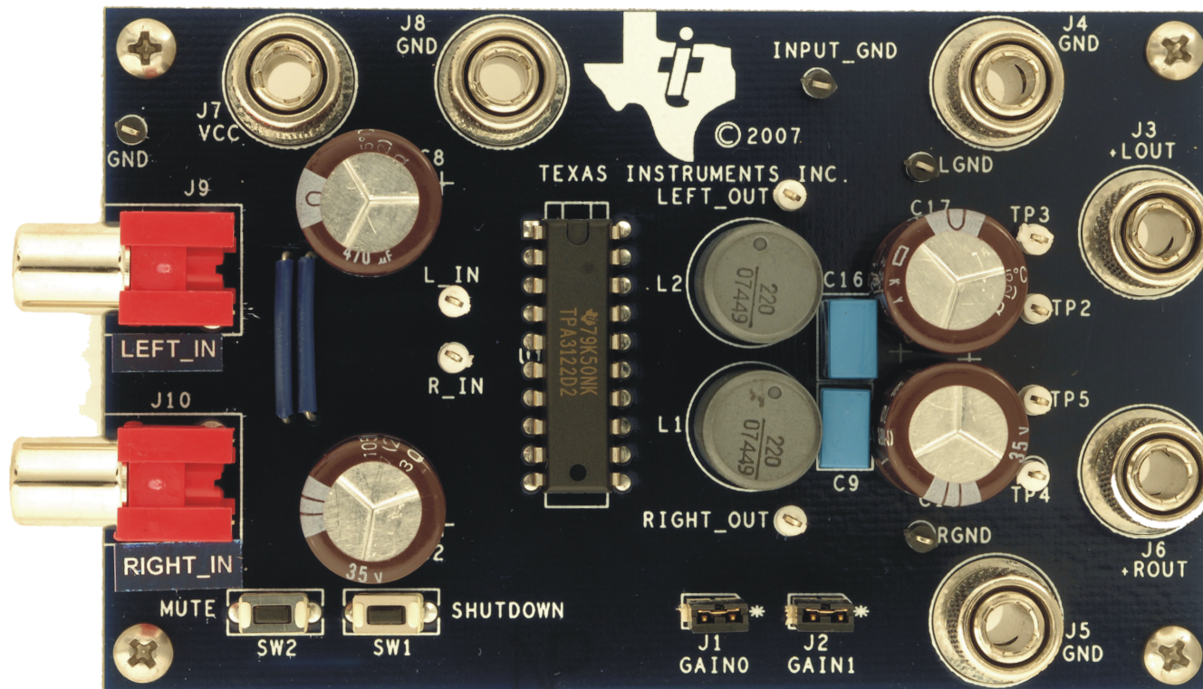
Figure 1. TPA3122D2 Audio Power Amplifier EVM - Top View
