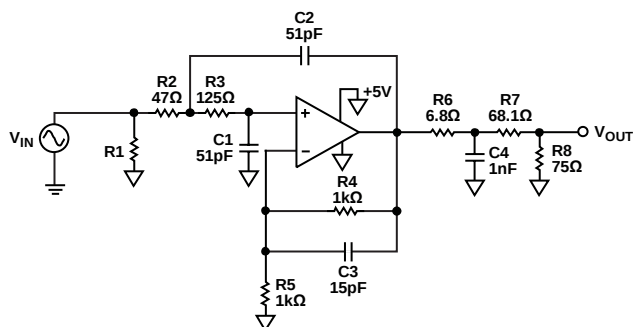
Figure 62. 15 MHz Video Reconstruction Filter Schematic
