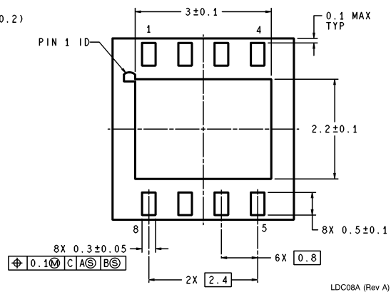
8-Lead LLP NS Package Number LDC08A
