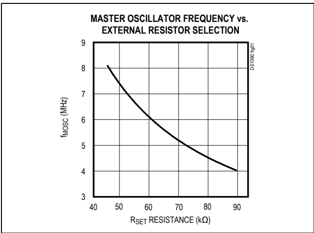
Figure 1. Master Oscillator Frequency
